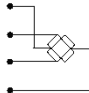
10VDC Strain Gauge Supply
