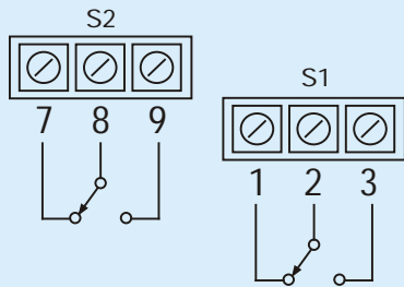
DigiRail - 2R Relay Output
